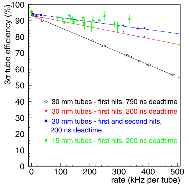
Fig. 5. 3\sigma single-tube efficiencies as function of the background rate. The green points show the measurements for the thin tubes. The efficiencies of the standard ATLAS drift tubes are taken from a previous measurement published in [11].
