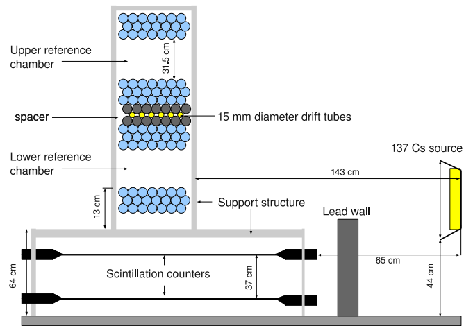
Fig. 1. Schematic drawing of the experimental set-up at the GIF.
