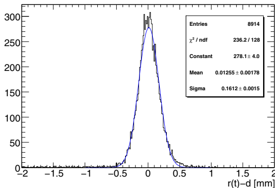
Fig. 4. Residual distribution at low counting rate.
