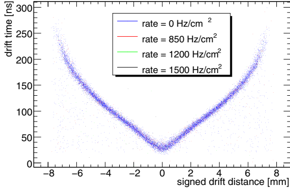
Fig. 3. Space-to-time relationship in 15 mm diameter tubes as a function of the counting rate. The sign of the drift distance indicates whether the anode wire was passed on its left or right.
