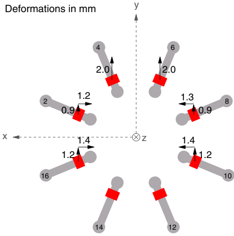
Fig. 3. Deformations of the barrel toroid at full field
