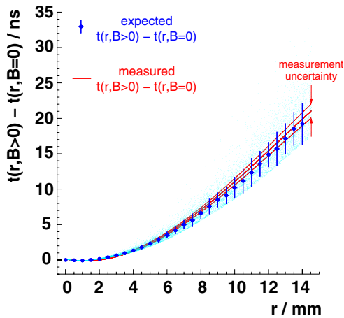
Fig. 10. Expected and measured change of the drift time in dependence of the drift radius for a chamber from the middle layer. The light blue dots represent the simulated time prolongation in all areas of the chamber. The spread of the dots is caused by the inhomogeneous field along the tubes. The filled circles with error bars are their mean value and RMS and the red line represents the measurement.
