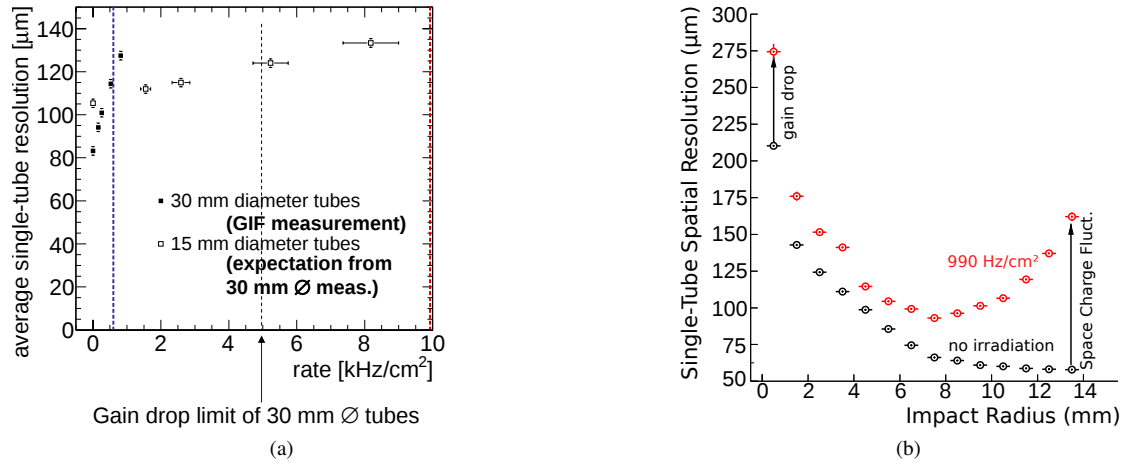
Fig. 1: Average spatial drift tube resolution as a function of the background counting rate in 15 mm and 30 mm diameter tubes (a) and spatial resolution as a function of the impact radius for tubes which were irradiated with a \gamma flux of 990 \text{Hz}/\text{cm}^2 compared to non-irradiated tubes (b).
