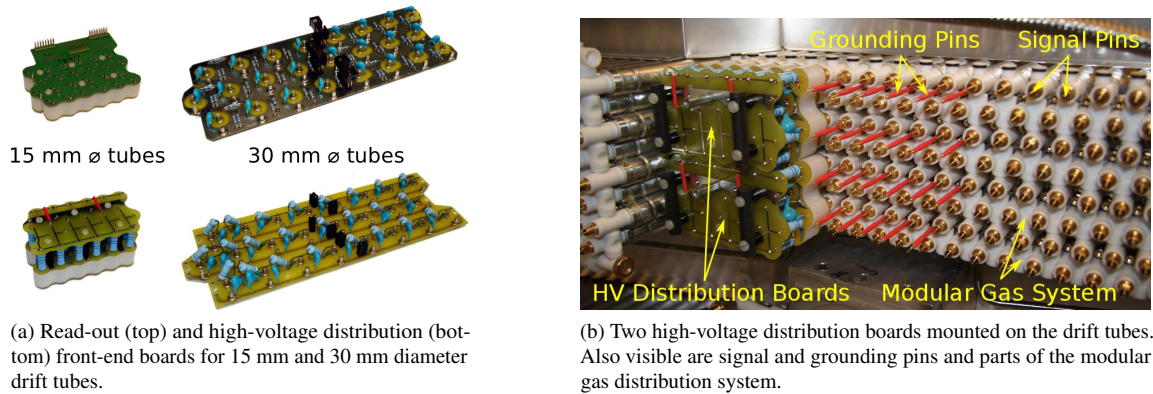
Fig. 3: Photographs of the high-voltage distribution and read-out front-end boards
