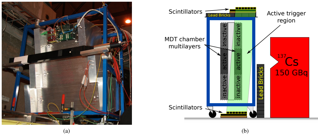
Fig. 4: Measurement setups (a) in a high energy muon beam at the H8 beam line and (b) at the Gamma Irradiation Facility at CERN. Scintillator detectors were used in both configurations for triggering on the beam and cosmic muons, respectively.
