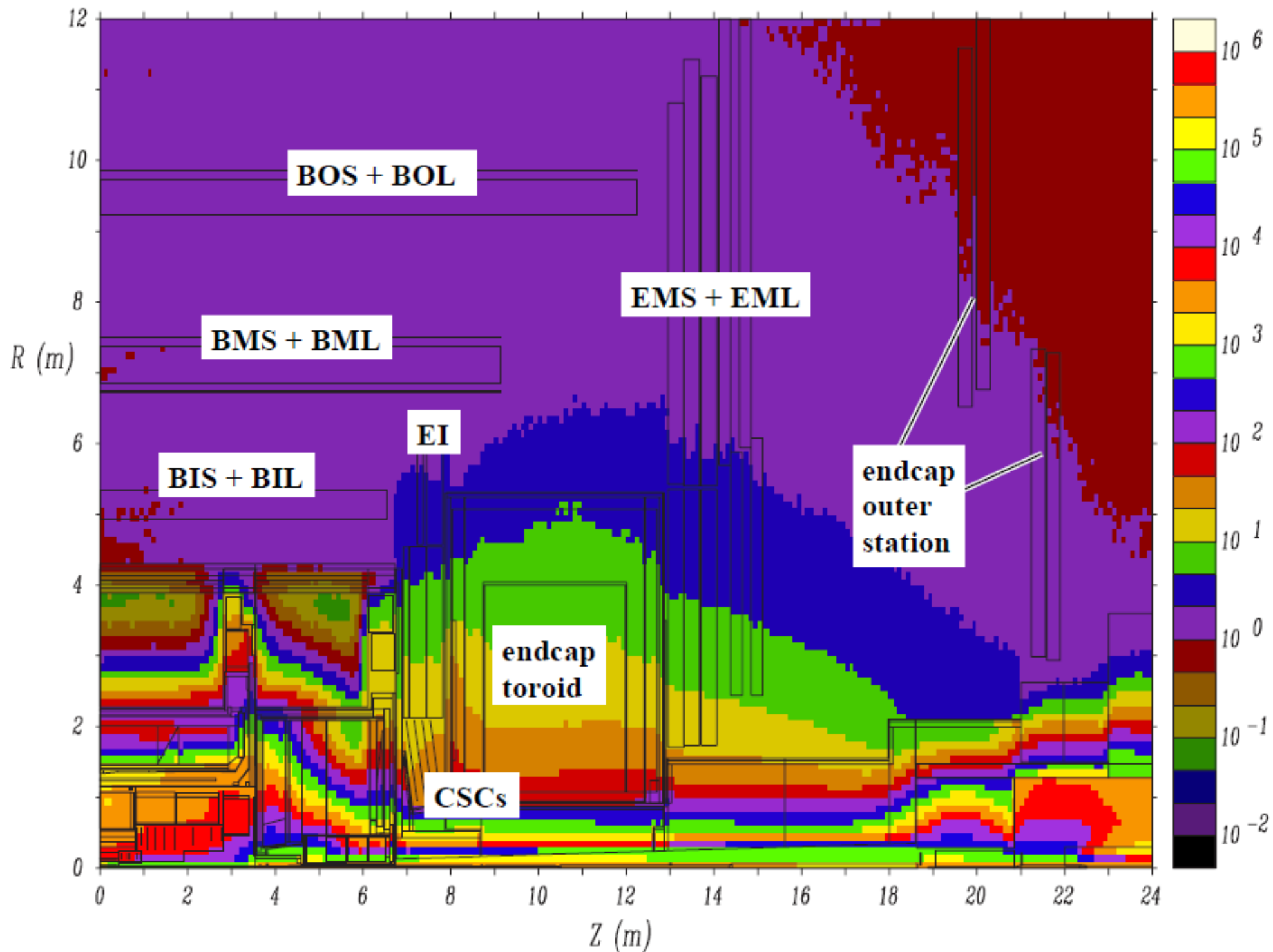
Jan03 Base (24620) - Photon Flux, KHz/cm**2
