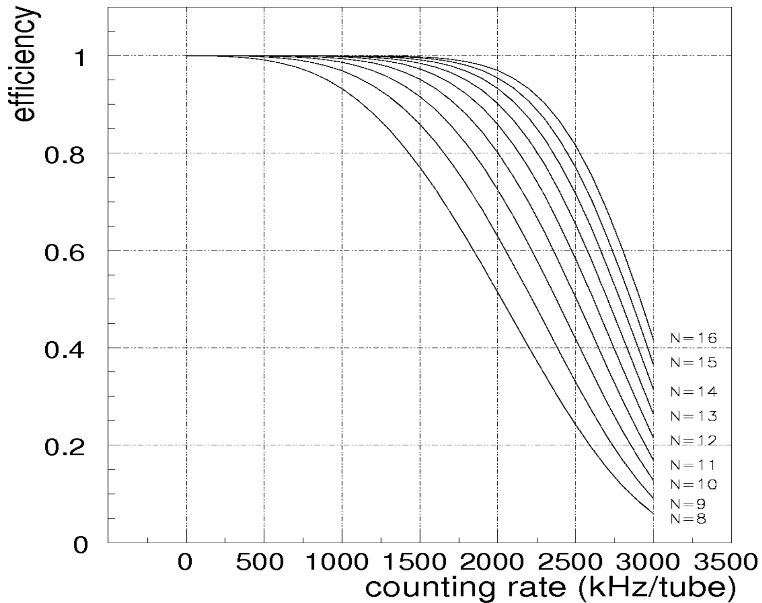
Segment reconstruction efficiency requiring at least 4 out of N hits
