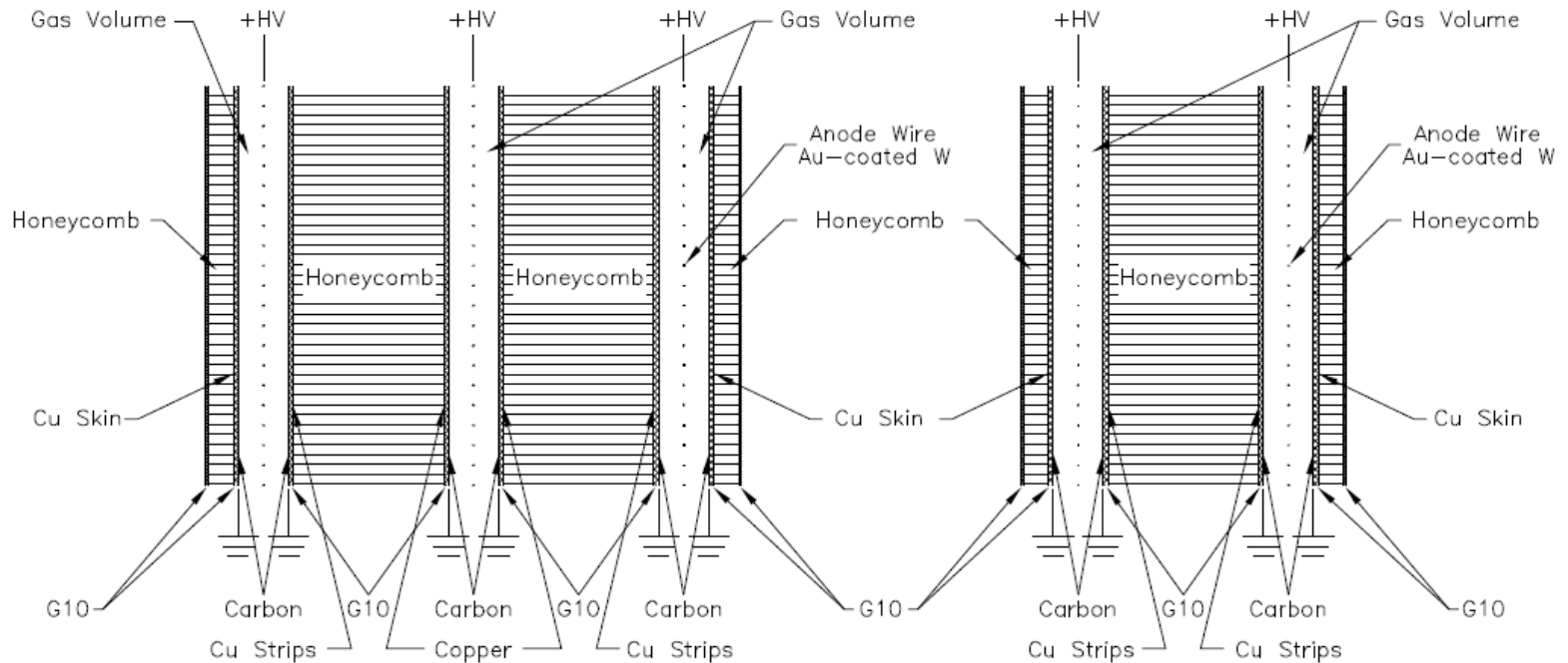
Figure 151. Cross-section of a TGC triplet and doublet module. The triplet has three wire layers but only two strip layers. The dimensions of the gas gaps are enlarged with respect to the other elements.
