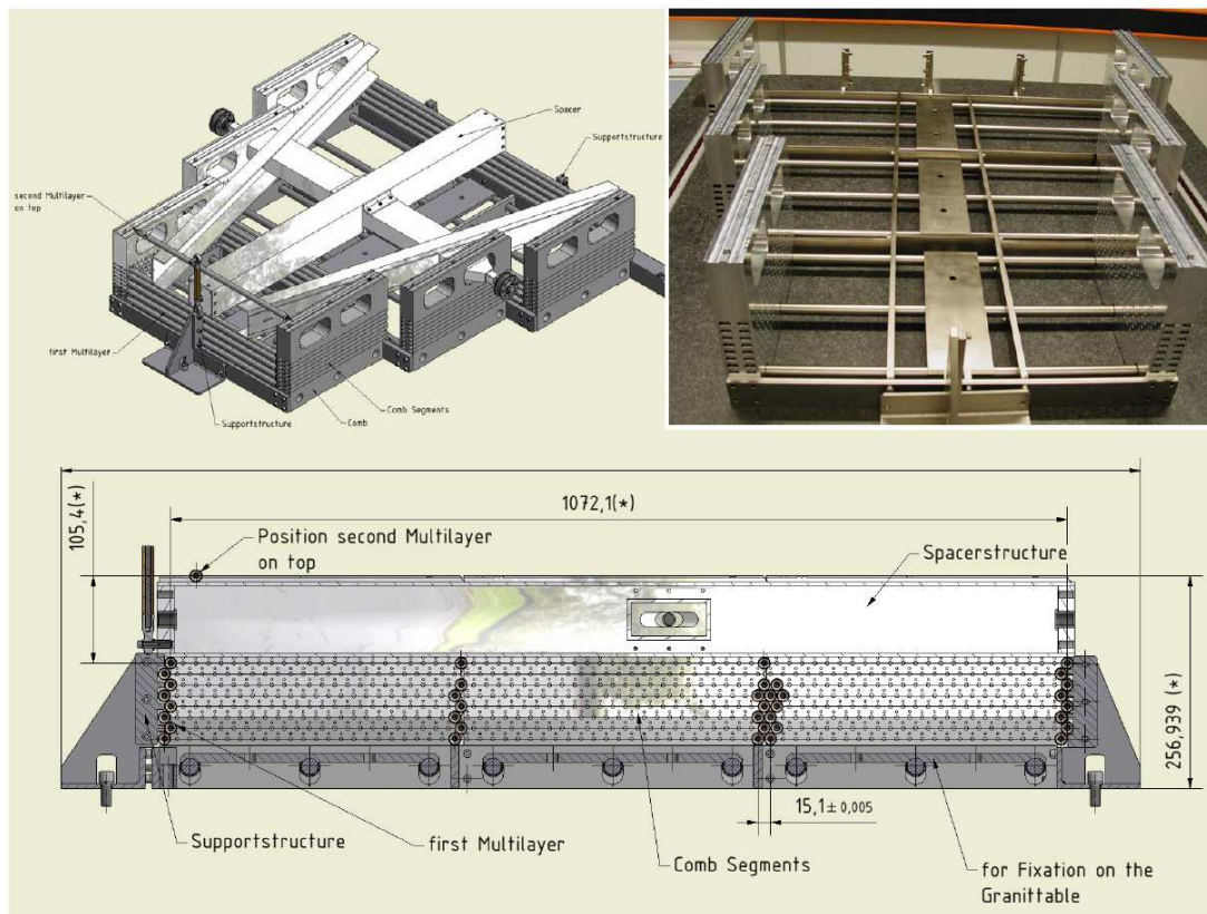
Figure 24: Assembly tooling for the sMDT chambers with precise positioning of the endplugs of the drift tubes holding the sense wires. The jigs are modular and adjustable for the construction of different chamber types. References for the precise mounting of the alignment sensor platforms with respect to the wires are part of the jig design.
