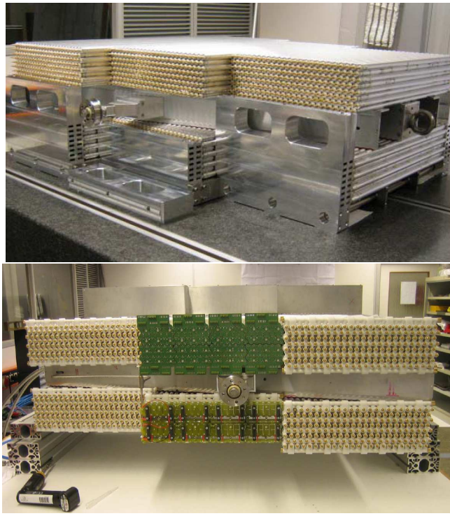
Figure 25: The sMDT prototype chamber during and after assembly, consisting of two multi-layers with 8 tube layers each, 72 tubes per layer and 1152 tubes in total.
