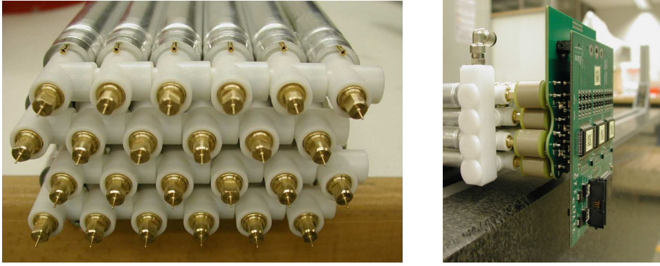
Figure 28: Left: The gas manifold for the Small tube chambers. The gas distribution is integrated into the endplug design. No gas bar with separate connections to each tube is needed. Right: The HV-coupling capacitors, housed in small plastic cylinders, are directly plugged onto the signal pins. In the next layer: signal distribution (“hedgehog”) and frontend electronics (“mezzanine card”).
