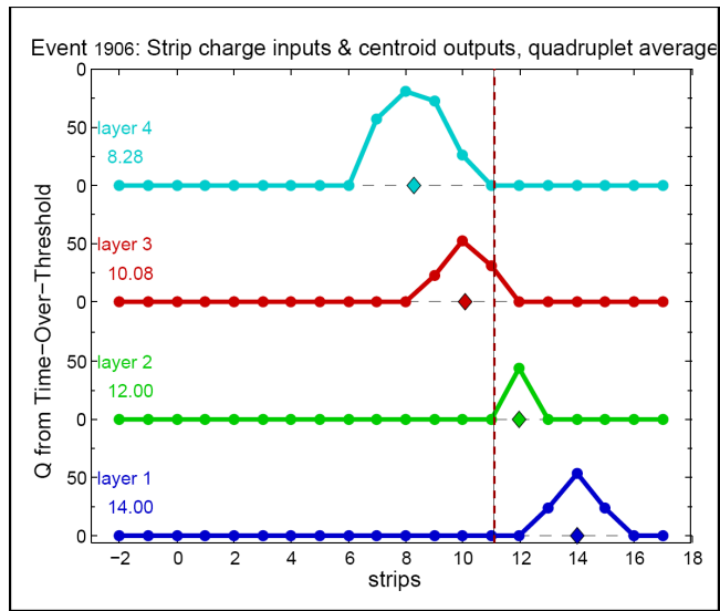
Figure 32: The four input strip profiles and the four calculated output centroids for a cosmic ray passing through a quadruplet. The centroid locations calculated by the demonstrator are on the left and are plotted as diamond symbols. The dashed line is the calculated average.
