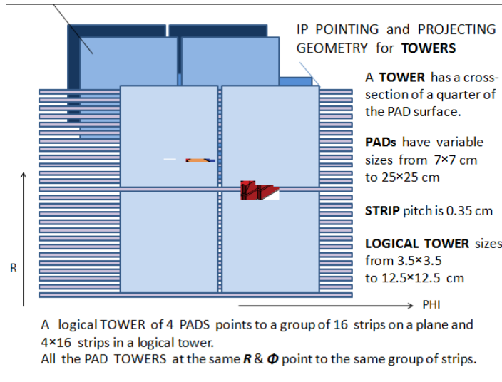
Figure 5: Schematics of Pad and strips arrangement (only 2 layers shown).
