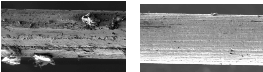
Figure 9: Deposits observed in the irradiated (left) and non-irradiated region of a wire.
