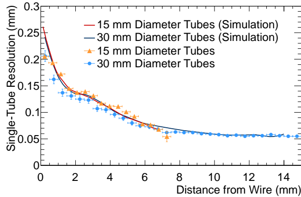
Figure 17: Spatial resolution of large and small tubes in the H8 test beam together with simulation results.
