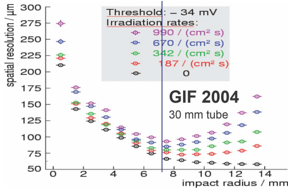
Figure 22: Dependence of the average spatial resolution of 30 mm diameter drift tubes on the background hit rate.
