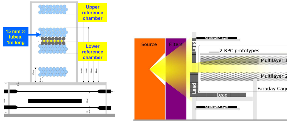
Figure 29: The test setup in the H8 test beam (left) and in the GIF (right).
