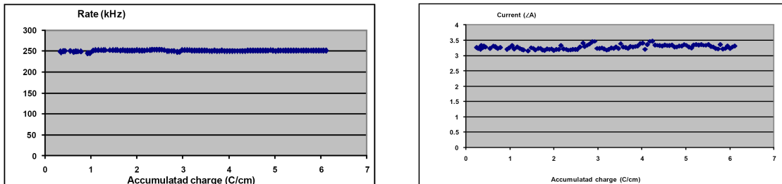
Figure 8: Counting rate and current as a function of the integrated charged in the detector.
