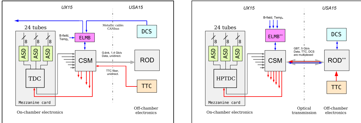
Figure 18: Schematic diagram of the present (left) and of the future MDT readout chain (right). Using the GBT in the new readout scheme improves the readout bandwidth and simplifies logistics, as TTC, Data readout and DCS are transferred over the same bi-directional link.
