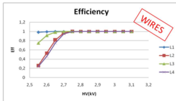
Figure 11: Plateau curve for each of the gaps used in the test, using the T-O-T method.
