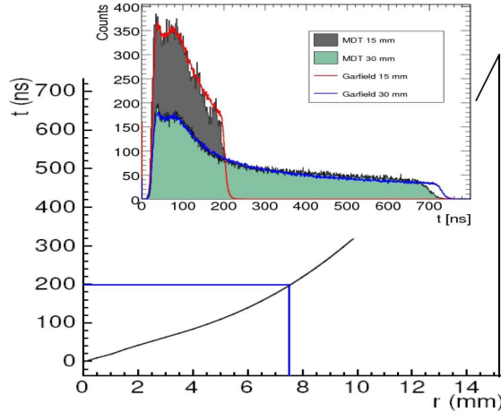
Figure 20: Space-to-drifttime ( r - t ) relationship of circular drift tubes operated with Ar:CO 2 (93:7) gas mixture at 3 bar.
