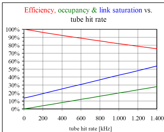
Figure 19: Green: Occupancy as a function of tube hit rate, assuming a dead time of 200 ns (equal to the maximum drift time) after each hit. Red: Resulting efficiency with the same dead time. Blue: Saturation of the mezzanine-to-CSM link, showing the base load of 15% due to the overhead of the transfer protocol at zero rate.
