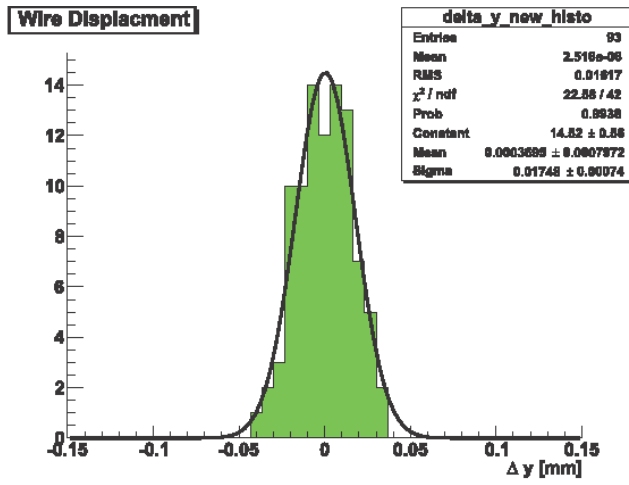
Figure 26: The accuracy of wire positioning in the prototype chamber is better than 20 \mu\text{m} rms.
