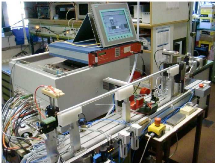
Figure 23: The semi-automated drift tube assembly station.
