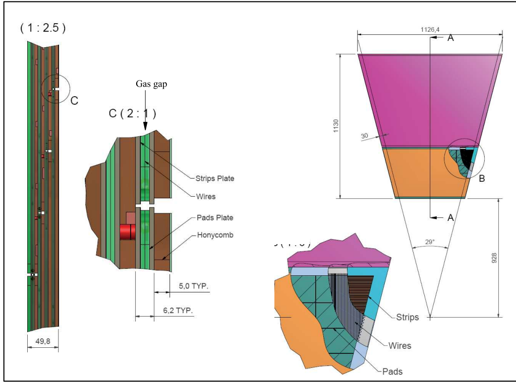
Figure 3: Schematics of the internal layout of a 4-layer TGC package, showing the pad-strip and wire readout for each gas-gap.
