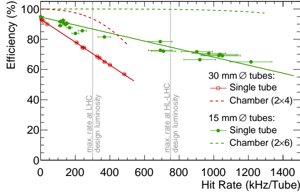
Figure 16: Efficiency versus background hit rate as measured at the GIF.
