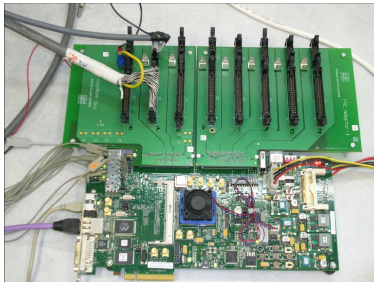
Figure 31: The trigger demonstrator board based on a commercial evaluation board (Xilinx ML605 with Virtex-6 FPGA). LVDS cables from eight TGC ASD modules are connected to the FPGA via custom mezzanine cards. These cards provide the required non-standard LVDS termination and merge power, threshold and test pulse lines from an external NIM module onto the cables to the ASDs. 64 strips and 44 pads are read out.
