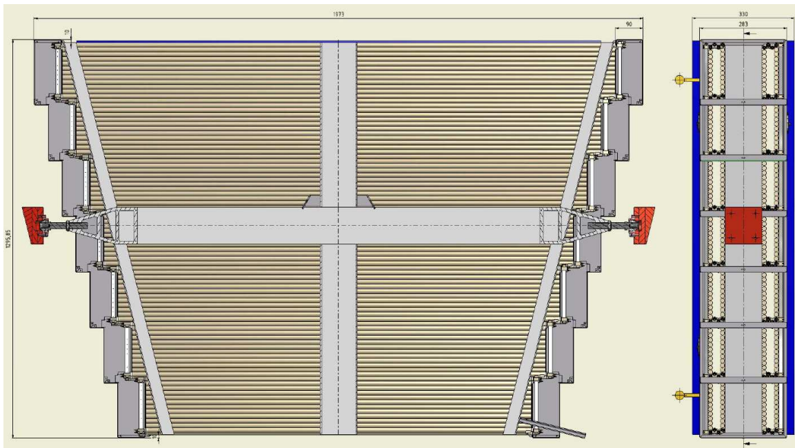
Figure 6: Small drift-tube chamber design for the new Small Wheels. The integration with the trigger chambers is also shown.
