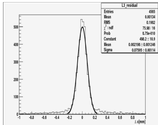
Figure 12: Typical residual for one of the layers with respect to the fitted line.
