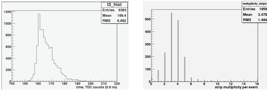
Figure 10: Left: Time difference between 3-out-of-4 pad trigger with respect to the beam scintillator in units of 0.8 ns. The FWHM is 11 ns. 99% of the distribution is within 25 ns. Right: Strip multiplicity for a MIP on a typical gas gap.
