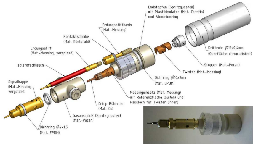
Figure 7: Exploded view of a drift tube with gas connection, signal and ground connection and encapsulated high-voltage decoupling capacitor.
