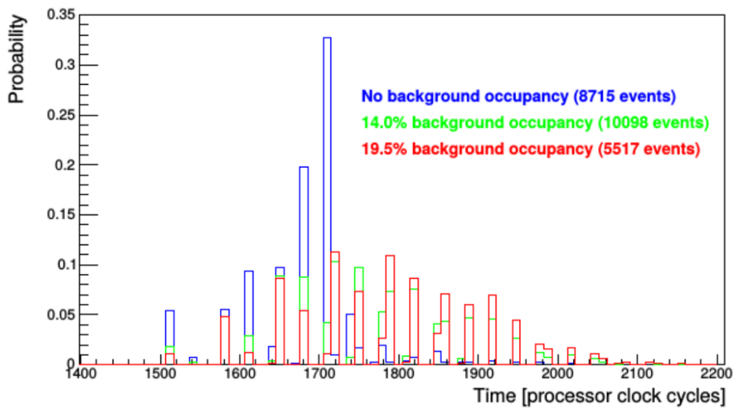
Figure 1: Processing time distribution for a fast track reconstruction algorithm for data acquired in CERN gamma irradiation facility.
