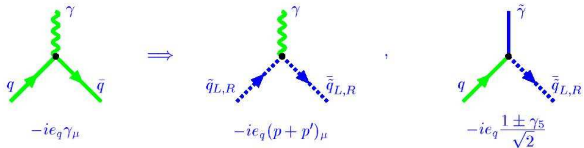
Fig. 12: Gauge-matter interaction
