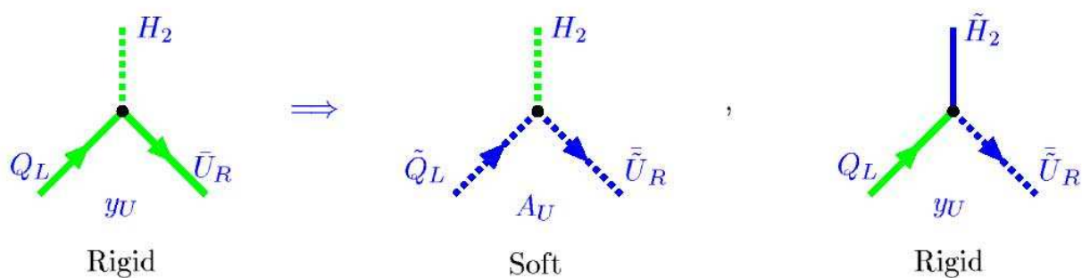
Fig. 14: Yukawa-type interaction
