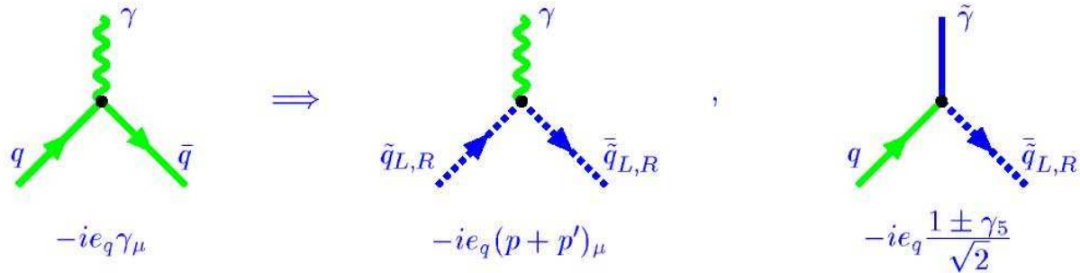
Fig. 12: Gauge-matter interaction
