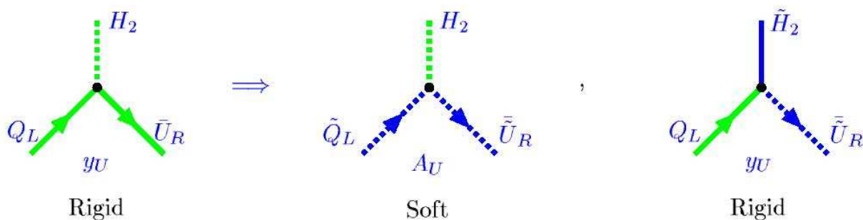
Fig. 14: Yukawa-type interaction
