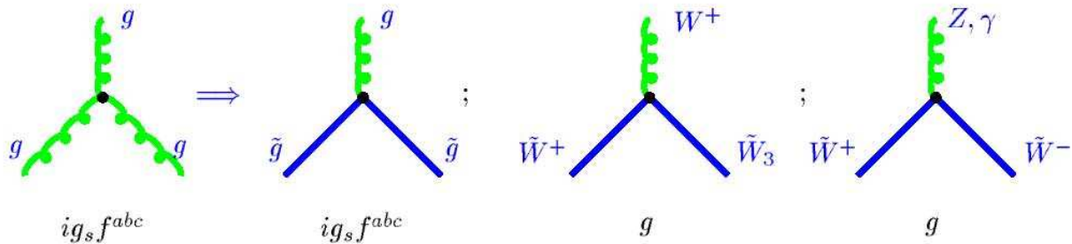
Fig. 13: Gauge self-interaction
