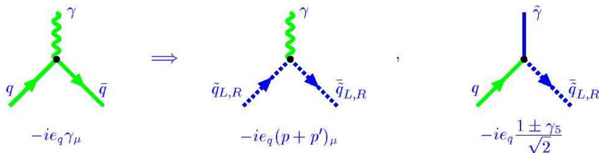
Fig. 12: Gauge-matter interaction
