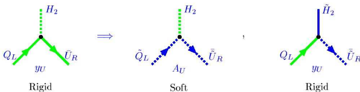
Fig. 14: Yukawa-type interaction
