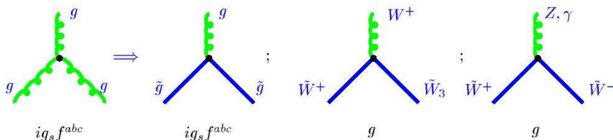
Fig. 13: Gauge self-interaction
