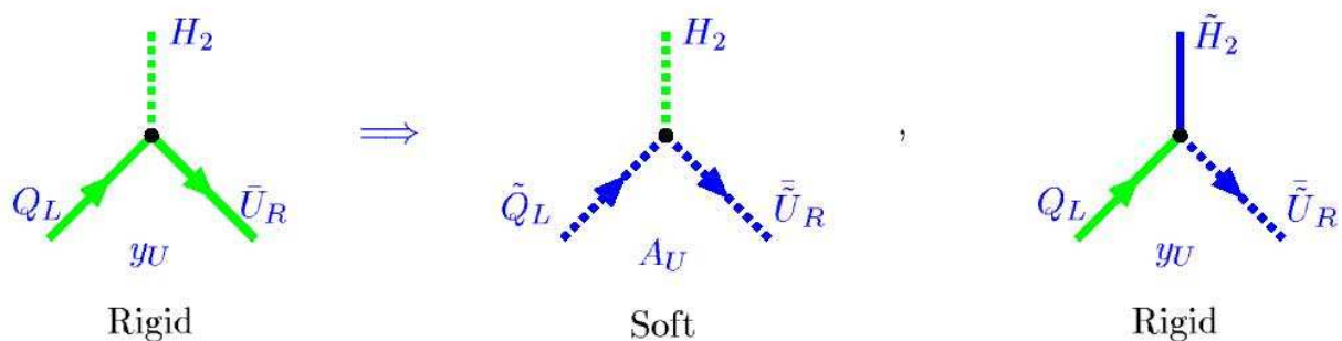
Fig. 14: Yukawa-type interaction
