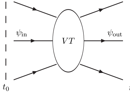
Figure 1: Schematic diagram of “in” and “out” states considered in high energy particle collisions.
