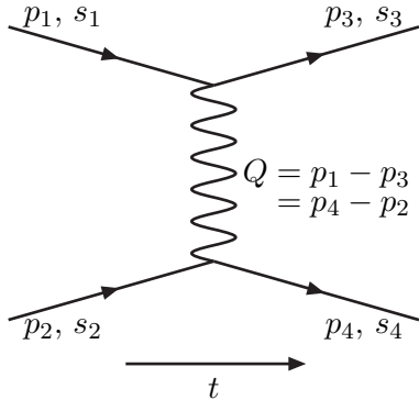
Figure 2: Diagram of first-order electromagnetic scattering of two non-identical fermions.
